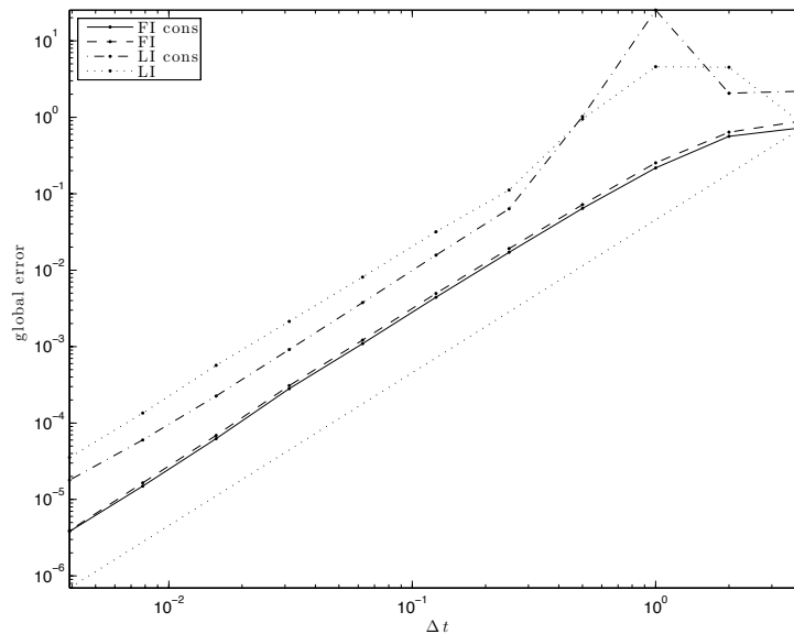
Figure 6.3: The global error at t = 8 for the schemes (1.2) (FI cons), (1.3) (LI cons), (6.3) (FI), and (6.4) (LI). The dotted line is a second order reference line.
