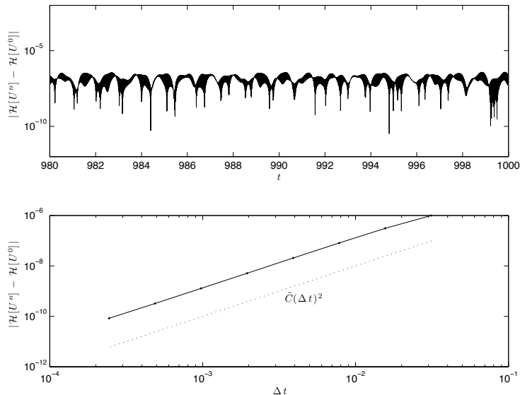
Figure 1.2: The error in \mathcal{H} as a function of the solution obtained by the linearly implicit scheme 1.3 as a function of t (top) and \Delta t (bottom). The dotted line is a reference line \tilde{C}(\Delta t)^2 .
