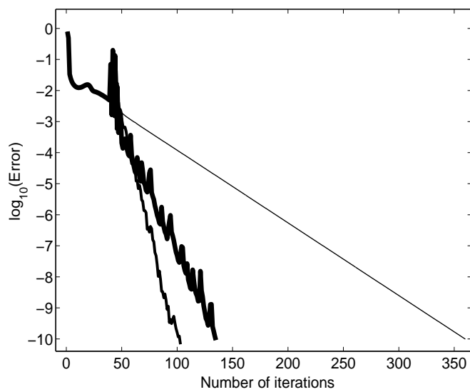
Figure 8: The evolution of the error in Example 4.3; in all cases, the application of (4.5) and/or acceleration is begun when the error norm reaches 5 \cdot 10^{-3} . Thin line: method (4.4) (no mode elimination); thick line: method (4.7) with s = 1 ; medium line: method (4.7) with s = 0.7 .
