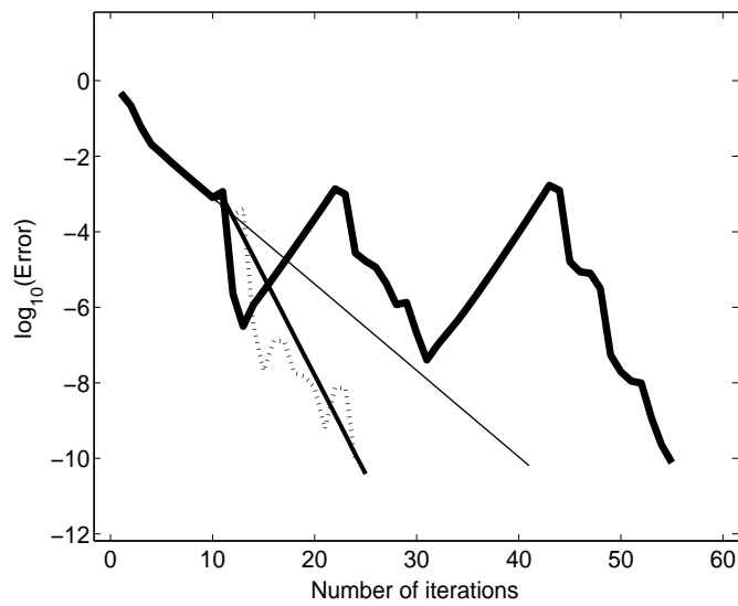
Figure 6: The evolution of the error in case (c) of Example 4.2. Thin solid: non-accelerated method (2.10); thick solid: method (3.7), (3.8) with s = 1 ; medium solid: method (3.7), (3.8) with s = 0.7 ; thick dotted line: Steffensen's method.
