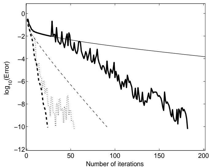
Figure 5: The evolution of the error in cases (a) and (b) of Example 4.2. Thin solid: non-accelerated method (2.10) for case (a); thick solid: method (3.7), (3.8) with s = 1 for case (a); thin dashed: non-accelerated method (2.10) for case (b); thick dashed: method (3.7), (3.8) with s = 1 for case (b); thick dotted line: Steffensen's method for case (b).
