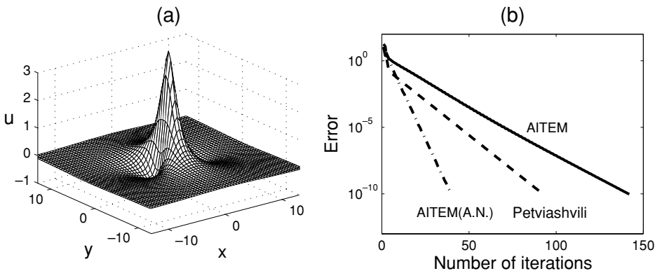
Figure 6. (a) A solitary wave in the KP equation (68) with \mu = 1 ; (b) error diagrams of the AITEM (with c = 1.4, \Delta t = 1.7 ), AITEM (A.N.) (with c = 1.4, \Delta t = 1.4 ) and the Petviashvili method for this solitary wave.
